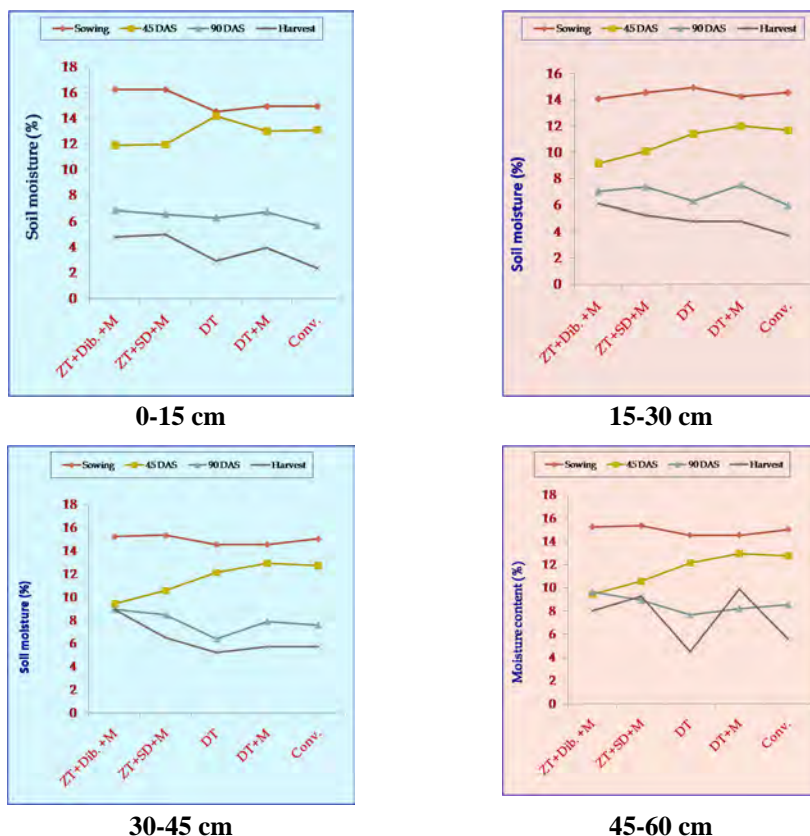
Fig 7. Soil moisture dynamics at different soil depth (0-15, 15-30, 30-45 and 45-60 cm) under conservation tillage (ZT: Zero tillage, Dib: Dabbling, M: Mulching, DT: Deep tillage, Conv.: Conventional tillage)
